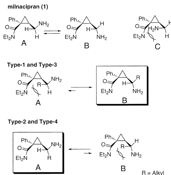
Figure 2. Conformational restriction of milnacipran by introducing an alkyl substituent at the 1'-position.
