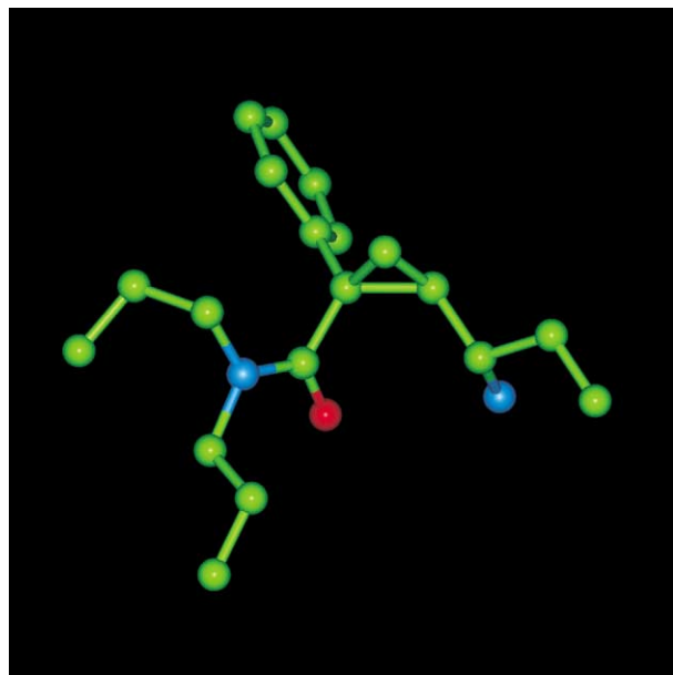
Figure 4. The MM2 calculation structure of 4d by simulated annealing method based on the NOE data.
