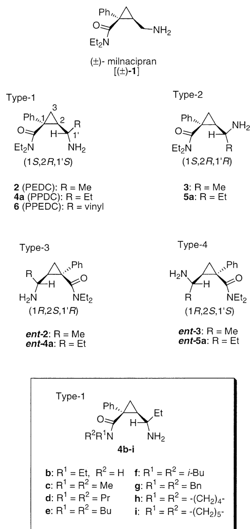
Figure 1. Milnacipran and its conformationally restricted analogues.
